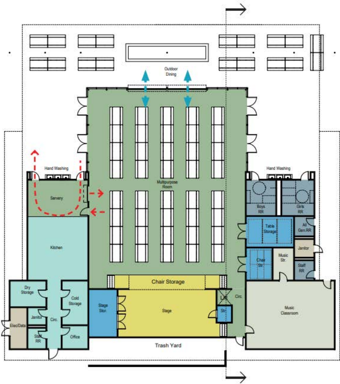
Floor Plan (Dining Capacity: ~300; Presentation Capacity: ~650)
